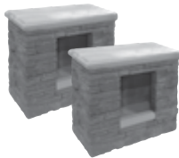
FIREPLACE WOOD BOXES 2'1¼"D x 3'3"W x 3'1"H per box Sold as a pair.
